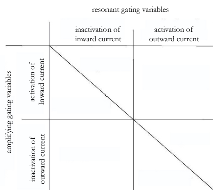
Figure. Any combination of one amplifying and one resonant gating variables results in a spiking model [3].
