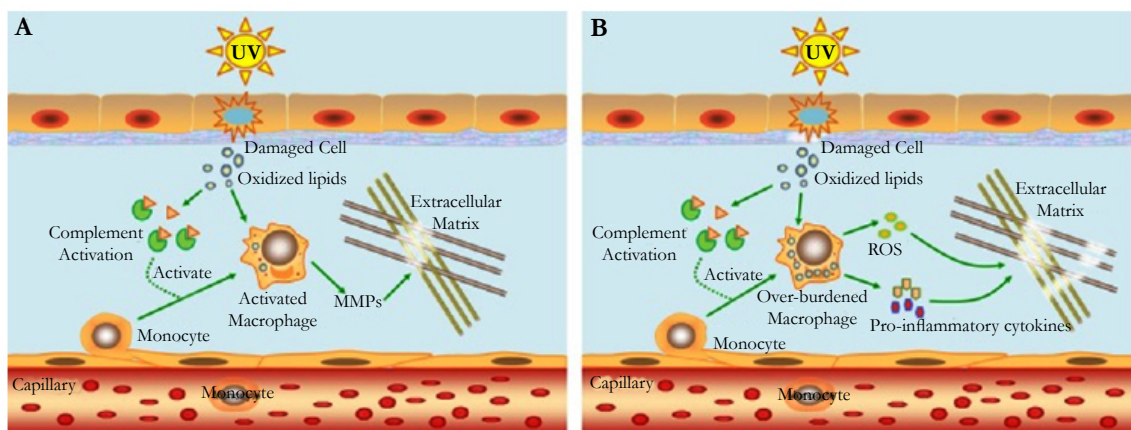
Figure 4. A model proposed to explain the mechanism of inflammaging in skin [11].
