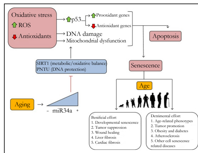
Figure 7. ROS-mediated senescence [42].
