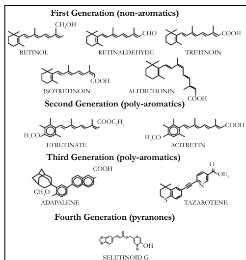
Figure 10. Chemical structures of retinoids [91-93].
