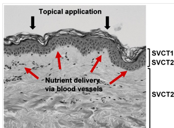
Figure 11. Delivery of nutrients to the skin [131].
